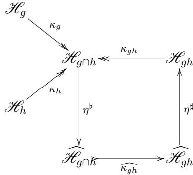
Figure 5.1: The multiplication diagram (again)
