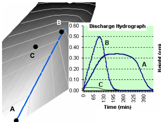
Figure 5. Mock watershed with output discharge hydrographs for channel (A,B) and terrain (C).
