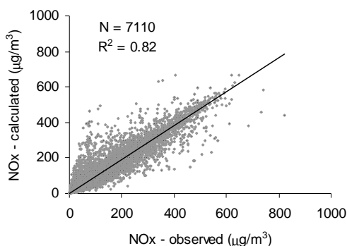
Figure 1. Comparison between measured and modeled concentrations of NO x in Riga (Valdemara street).
