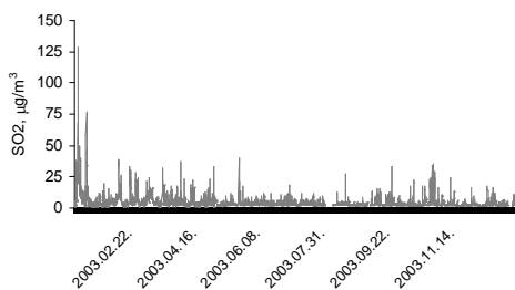
Figure 3c. Time series of SO 2 hourly concentrations in Riga: January-December 2003.
