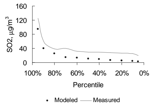
Figure 4c. Percentiles of SO 2 concentration in Riga: January-December 2003.
