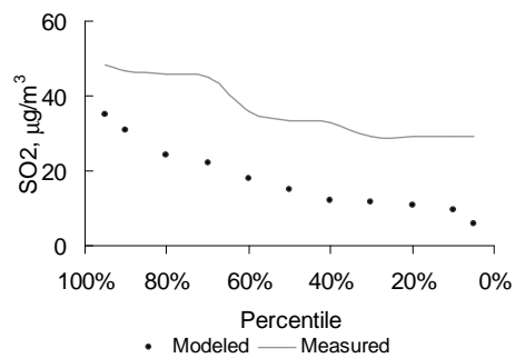
Figure 4b. Percentiles of SO 2 concentration in Riga: January-December 2002.
