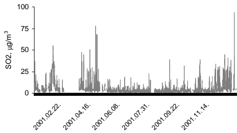
Figure 3a. Time series of SO 2 hourly concentrations in Riga: January-December 2001.
