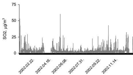
Figure 3b. Time series of SO 2 hourly concentrations in Riga: January-December 2002.
