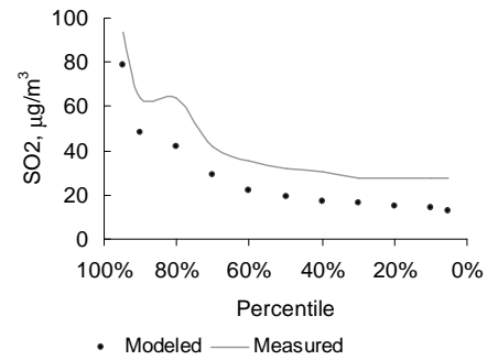
Figure 4a. Percentiles of SO 2 concentration in Riga: January-December 2001.
