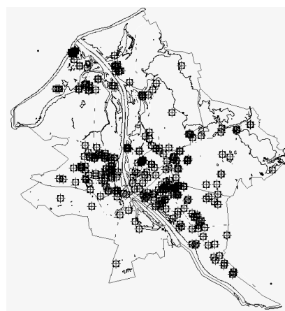
Figure 2. Location of SO 2 sources in Riga city (scale 1:40 000) .
