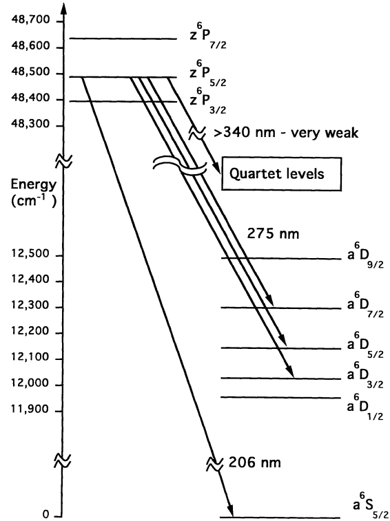
FIG. 2.—Partial Grotrian diagram showing the decay of the z^6P^{\circ}_{5/2} level of Cr II with approximate vacuum wavelengths. The unspecified quartet levels to which transitions have been observed include the a^6D_{3/2} , a^6D_{5/2} , a^6D_{7/2} , a^4P_{5/2} , and b^4P_{3/2} levels (Kiehl 1951).
