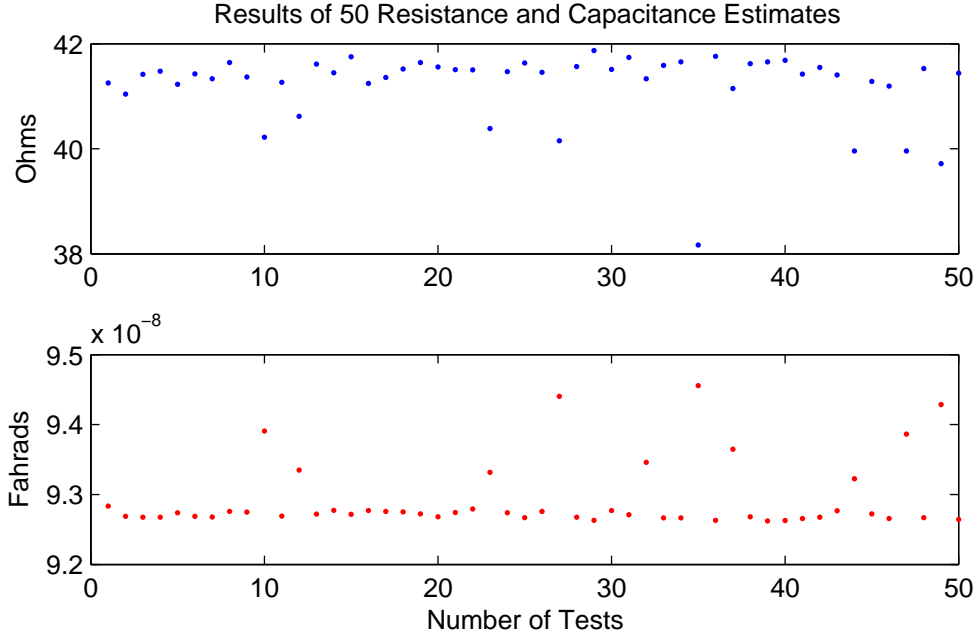
Figure 4.14: Results of 50 estimations of R_l and C_l without any load changes over the course of the test.
