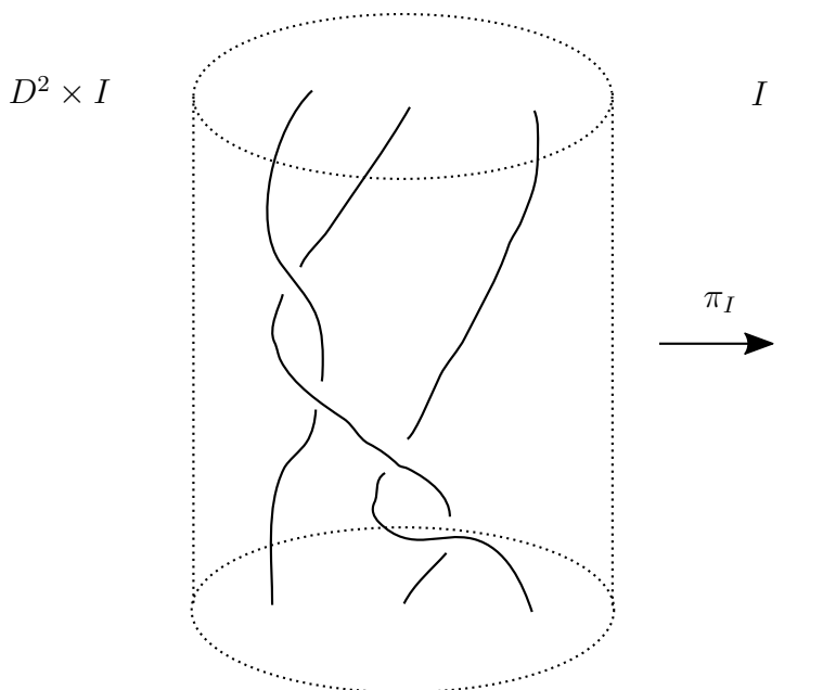
Figure 2.1: Topological braid in D^2 \times I .
