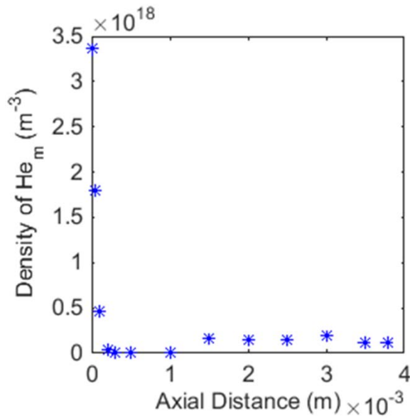
Figure 4-2 : Experimentally measured helium metastable atom densities in a DC glow discharge. The 0 point on the graph corresponds to the tip of the high voltage pin electrode. Error bars for these measurements are smaller than the data markers.
