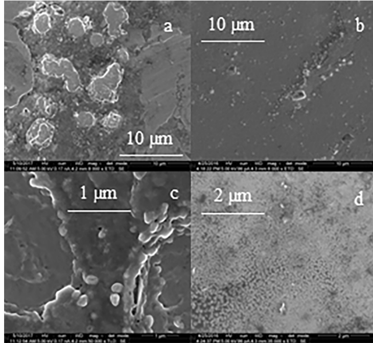
Figure 3-5 : SEM images of an unpolished copper surface exposed for 300 seconds to a pure argon discharge (a and c) and a H 2 /Ar discharge (b and d).
