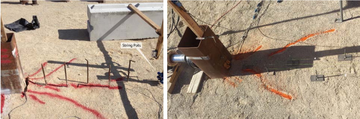
Figure 4-3: String Potentiometers in Place during Testing
