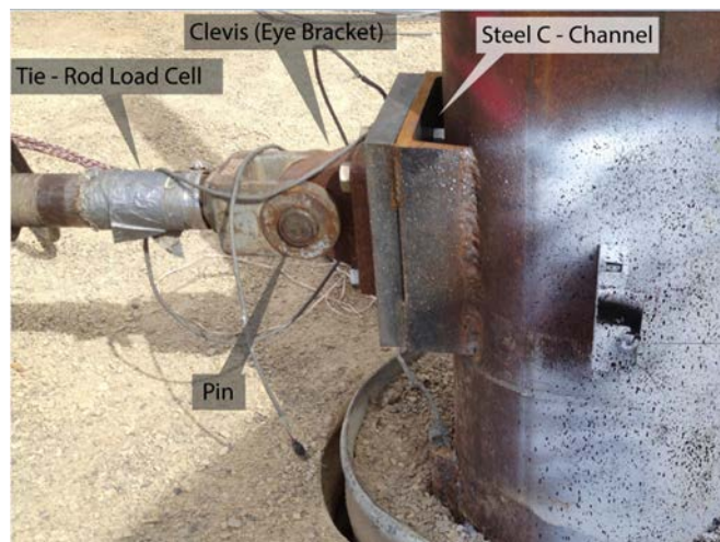
Figure 4-2: Pin Connection
