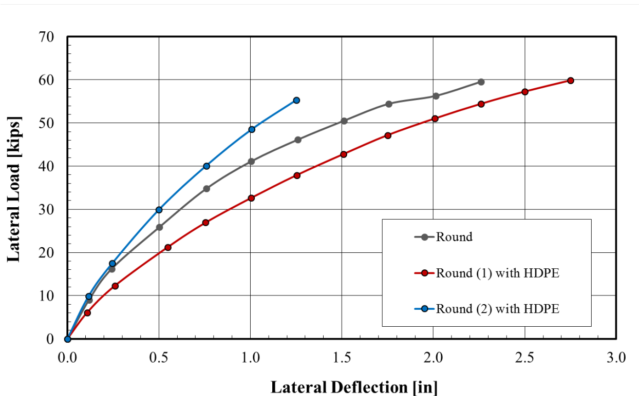
Figure 5-4: Load Test Results for Round Piles with HDPE Sheeting
