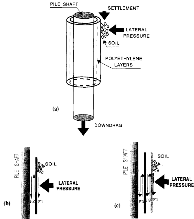
Figure 2-12: Plastic Sheeting for Downdrag Reduction: (a) Schematic; (b) One plastic Layer; and (c) Two Plastic Layers (After Caliendo and Tawfiq, 1995)
