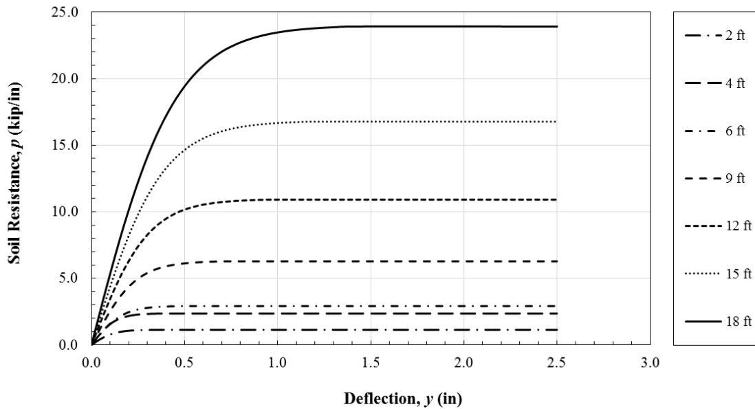
Figure 6-8: P-y Curves at a Specified Depth for a Round Pile
