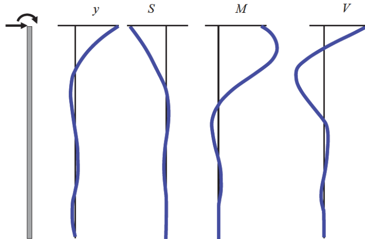
Figure 2-1: Deflection, Slope, Moment and Shear for a Pile Subject to Lateral Loading (After Isenhower and Wang, 2015)
