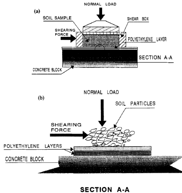
Figure 2-13: Direct-Shear Test on Concrete-Polyethylene-Soil Samples: (a) Full View; and (b) Section A-A (After Caliendo and Tawfiq 1995 page 7)
