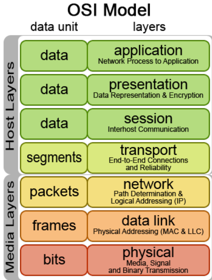
Figure 2-1: OSI Model
