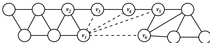
Figure 4.3: The completion of G - v to a 2-path
