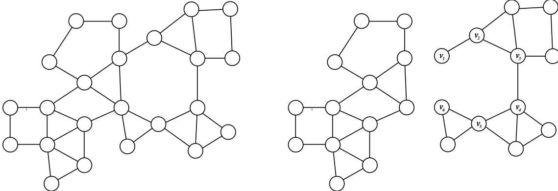
Figure 5.1: A 2-connected outerplanar graph with a particular 2-separation
