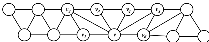
Figure 4.2: A labelled 2-path G
