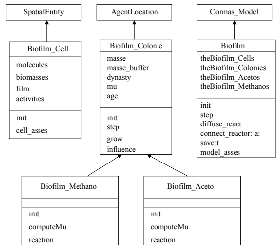
Figure 2. Model Architecture
