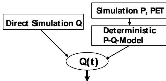
Figure 3. Runoff generation
