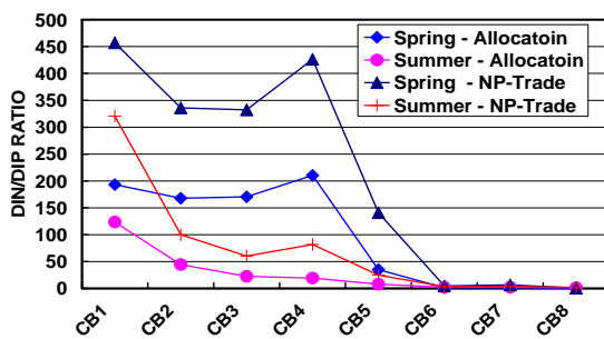
Figure 8. DIN/DIP ratio.
