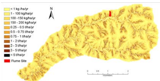
Figure 8: Predicted hillslope erosion of fine sediment which reaches streams in the Weany Creek catchment
