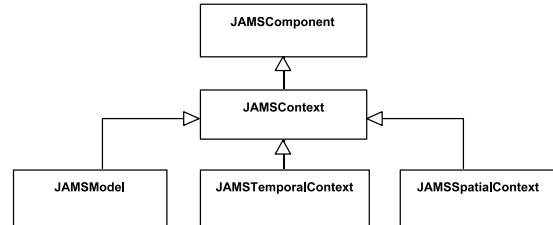
Figure 6: JAMS component hierarchy
