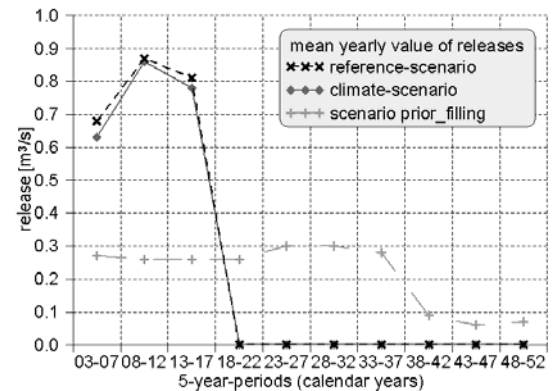
Figure 8. Water releases from the reservoirs Bautzen and Quitzdorf for filling of mining pits
