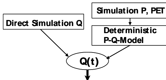
Figure 3. Runoff generation
