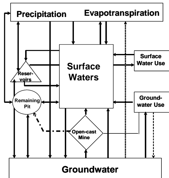
Figure 1. Water management scheme
