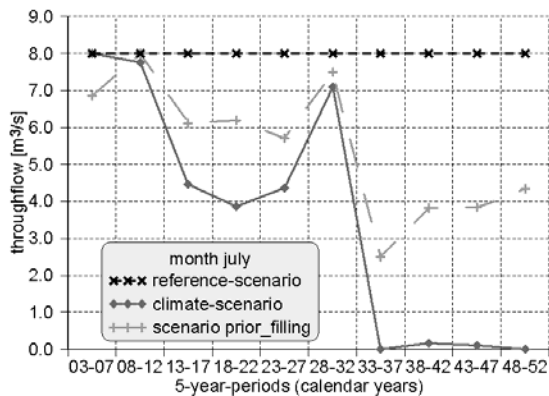
Figure 7. Discharge at inflow gauge to Berlin (Grosse Tränke/Spree river)
