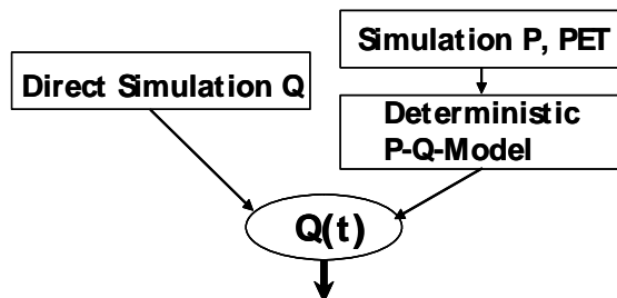
Figure 3. Runoff generation
