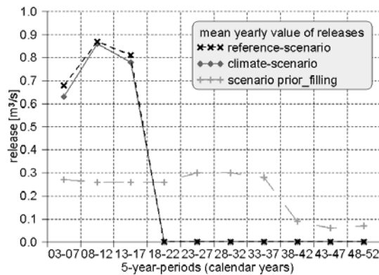
Figure 8. Water releases from the reservoirs Bautzen and Quitzdorf for filling of mining pits
