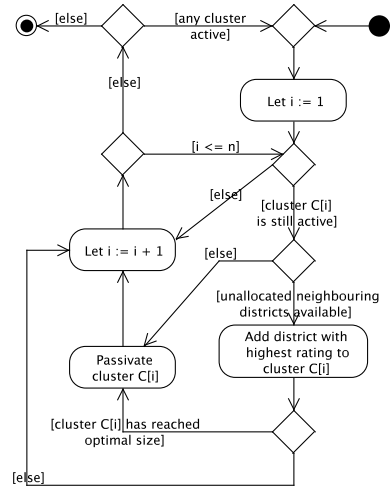
Figure 2: UML activity diagram of the basic cluster algorithm
