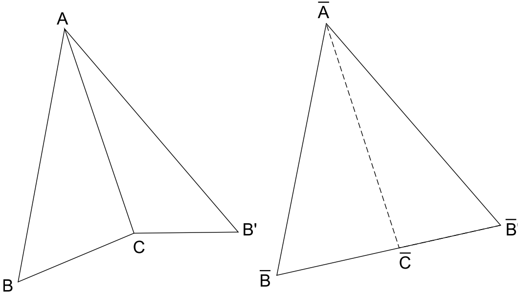
Figure 2.1: Alexandrov's Lemma
