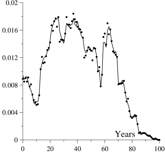
Figure 1. Distribution of men over age (line - statistical data, dots - model distribution).
