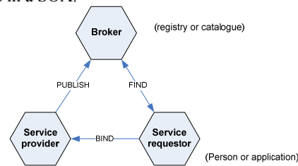
Figure 1. The publish, find, bind pattern
