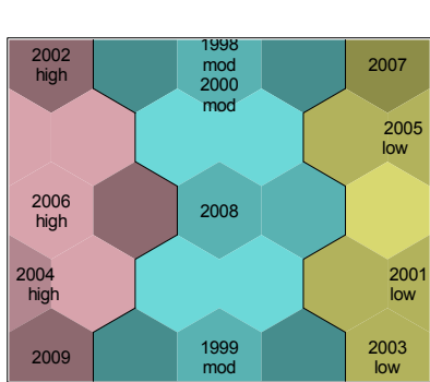
Figure 3 a: SOM components of monthly total GDD (base 10°C) and total frost days clustered based on vineyard annual yield ratings, left to right high, moderate, low yield . L: linear, NL: nonlinear and I: inverse correlation to yield class. ** regression and *** discriminant predictors. b: SOM of yield and monthly climate variables as in figures 1 and 2a. c: Results of regression analysis, yield rating against climate variables.
