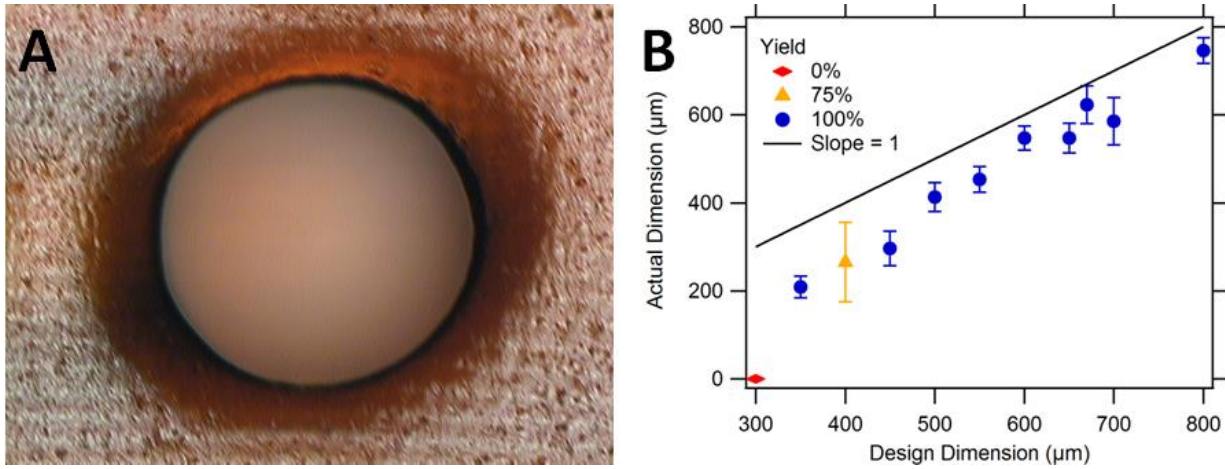
FIG. 4. Vertical cylindrical channel fabrication, repeatability, and yield. (A) Top view of a designed 650 \mu\text{m} cylindrical channel. The measured diameter of the channel is 606 \mu\text{m} . (B) Actual (measured) cylindrical channel size as a function of the designed size. Successfully printed open channels (yield) as a function of the designed cylinder diameters. Error bars denote standard deviation based on measurement of four channels (300-450 \mu\text{m} holes) or eight channels (500-800 \mu\text{m} holes).
