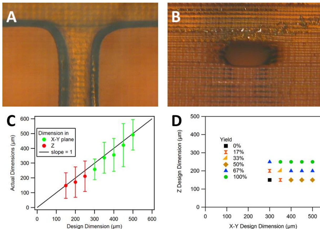
FIG. 3. Horizontal channel fabrication, repeatability, and yield. (A) Top view and (B) side view of a flow channel with designed cross section size of 350 \mu\text{m} \times 250 \mu\text{m} . The measured cross section of the fabricated flow channel is 316 \mu\text{m} \times 217 \mu\text{m} . (C) Average actual (measured) flow channel size as a function of the designed size (error bars show standard deviation based on measurement of 8 samples). (D) Yield as a function of the designed X-Y and Z dimension sizes for 8 devices where yield represents the frequency of a successfully printed open channel.
