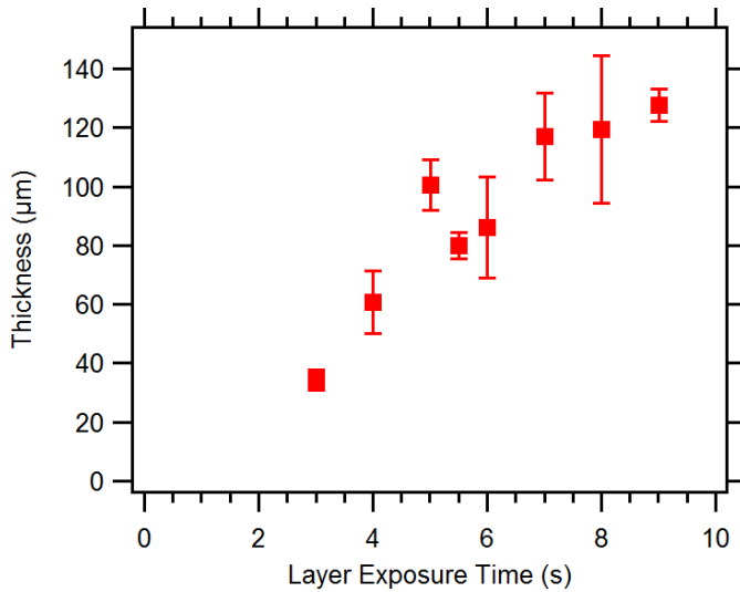
FIG. 5. Measured membrane thickness as a function of layer exposure time. In the design, the membrane thickness is specified as a single 3D printed layer. Error bars for data points at 3 seconds or greater exposure time represent standard deviation based on measurement of 4 to 9. There are no error bars for the 3 second data point, which is the average of two samples.
