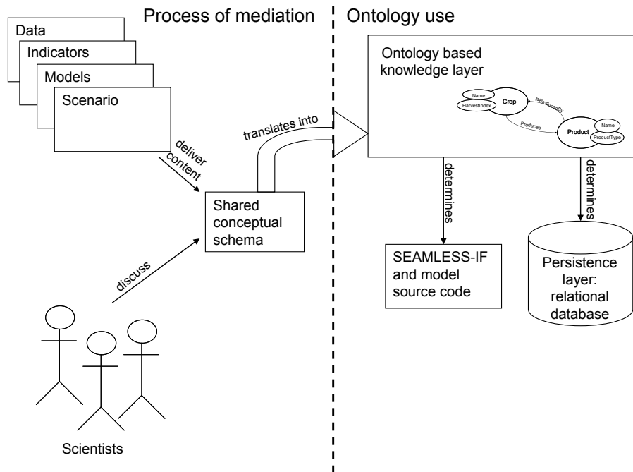
Figure 2. Process of ontology mediation (left side) and ontology use (right side).
