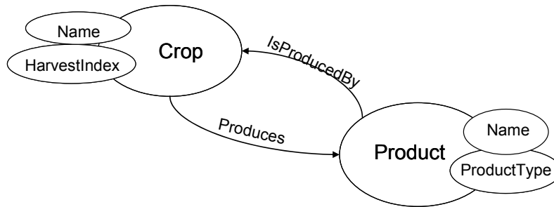
Figure 1. a part of an ontology showing two concepts (in ovals; Crop and Product ), their relationships (uni-directional arrows; relationship as Crop Produces Product and relationship as Product is-produced-by Crop ) and their data-properties ( Name for Concept Crop and Product , Producttype only for Concept Product and HarvestIndex only for concept Crop ).
