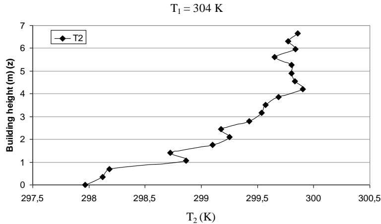
Figure 8. Central distribution of temperatures T_2 in the building
