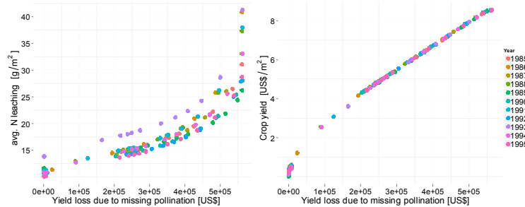
Figure 5. External effects by pollination on crop yields for the trade-offs using optimized landscapes case study. The different colours represent the simulation results for the different years.
