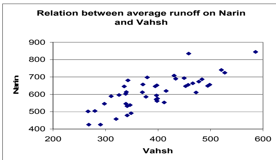
Figure 4. Relationship between annual water discharge at the cross-sections of the inflow to the Nurek reservoirs and Toktogul reservoirs ( R = 0.72 ) for the last 50 years.
