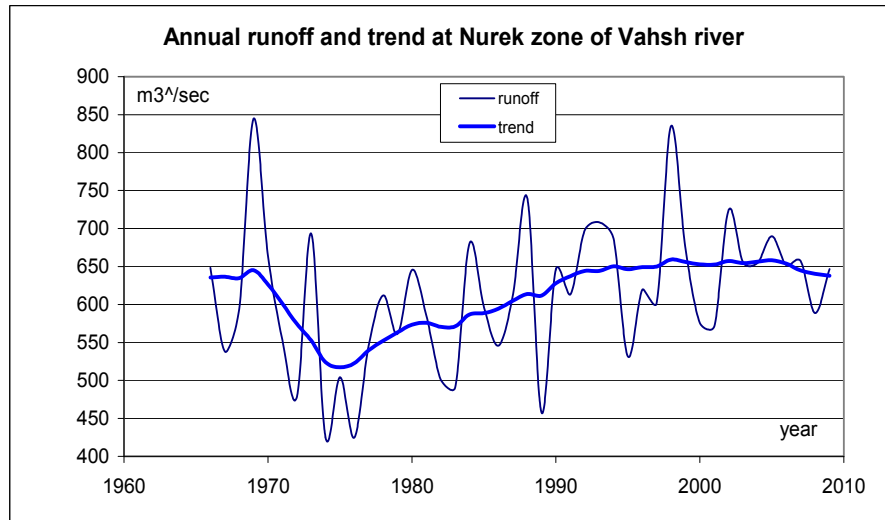
Figure 7. Historical data of the inflow in the Nurek reservoir and the trend for the last 50 years.
