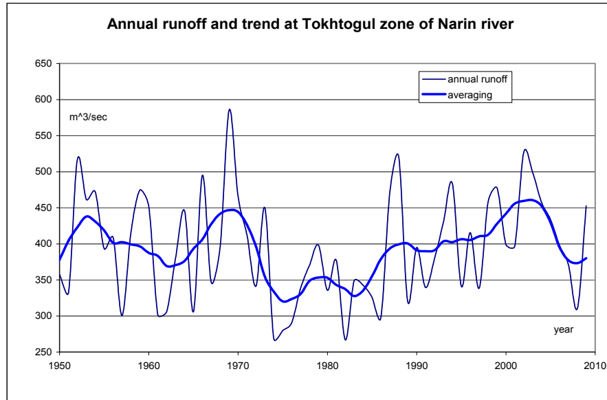
Figure 6. Historical data of the inflow in the Tohktogul reservoir and the trend for the last 60 years (moving averaging).
