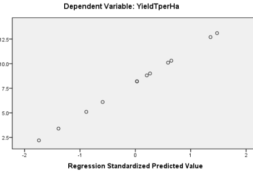
Figure 3 a: SOM components of monthly total GDD (base 10°C) and total frost days clustered based on vineyard annual yield ratings, left to right high, moderate, low yield . L: linear, NL: nonlinear and I: inverse correlation to yield class. ** regression and *** discriminant predictors. b: SOM of yield and monthly climate variables as in figures 1 and 2a. c: Results of regression analysis, yield rating against climate variables.
