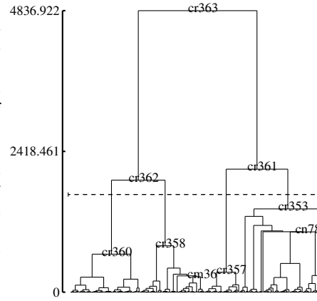
Figure 1: Dendrogram [\tau_{Lj3,R2}^{EnW,G}] .
