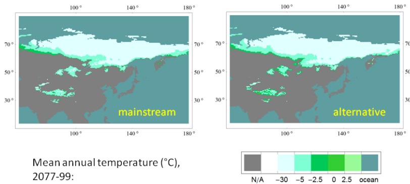
Figure 2. Mean annual temperatures in the permafrost regions (i.e., where \text{MAT} < -5^{\circ}\text{C} in present) as projected by the end of this century for SRB1 scenario: left pane – mainstream projection, right pane – alternative projection. Data source: outputs of sixteen climate models available at IPCC DDC. Method: inference tool of Carbon Sink Archives .
