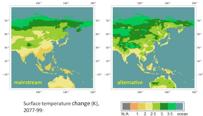
Figure 1. Anomalies in mean annual temperatures in the end of this century projected for SRB1 scenario: left pane – mainstream projection, right pane – alternative projection. Data source: outputs of sixteen climate models available at IPCC DDC. Method: inference tool of Carbon Sink Archives .
