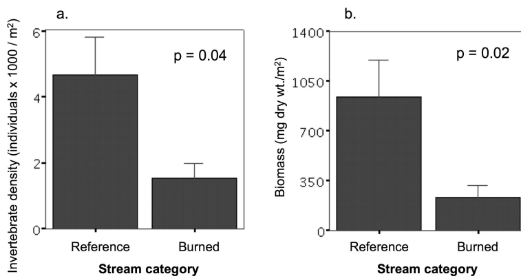
Fig. 2. Density (individuals \cdot 1000 \text{ m}^{-2} ) and biomass (mg dry weight \cdot \text{m}^{-2} ) of benthic macroinvertebrates in reference and fire-affected streams 2 years after fire (summer 2004). Error bars represent one standard error and, n = 5 streams per category. Data were log-transformed prior to statistical analyses.
