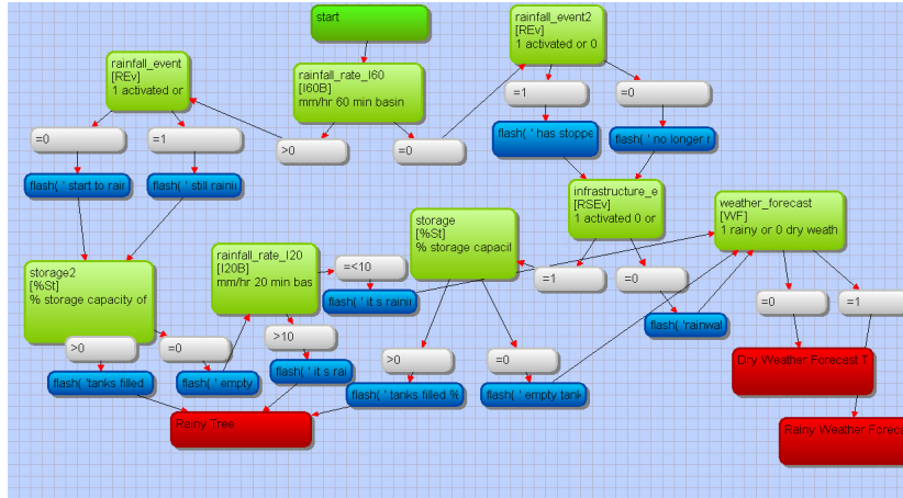
Figure 2. Decision tree for rain type diagnosis
