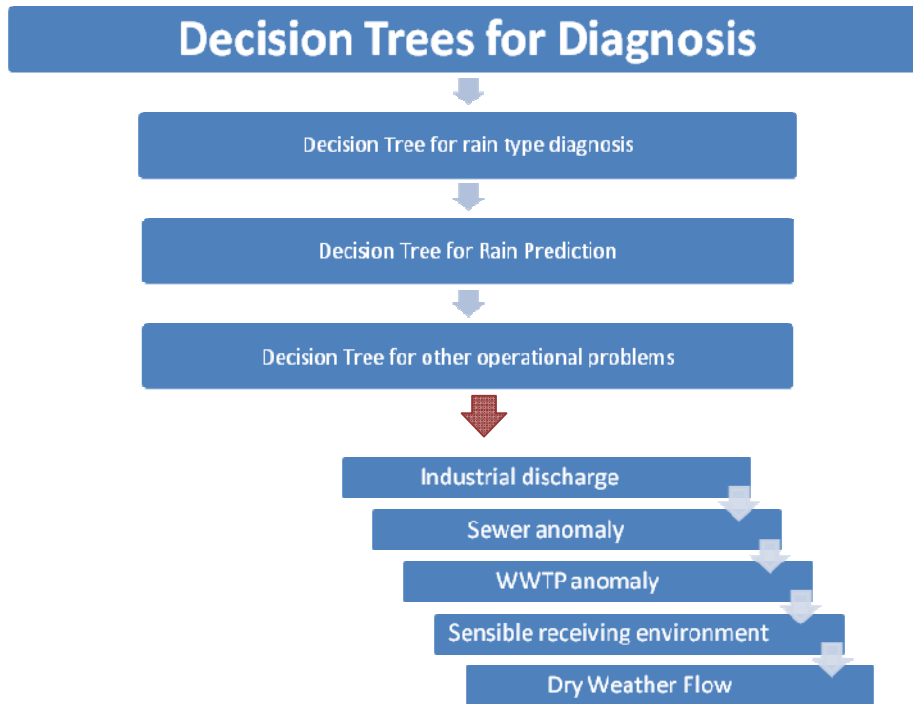
Figure 1. Hierarchy of decision trees for diagnosis
