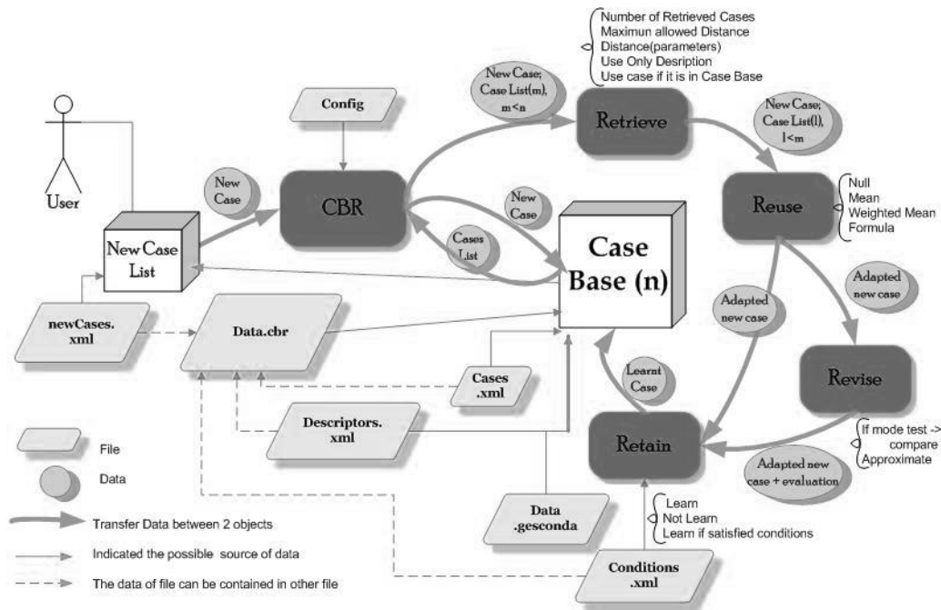
Figure 1: CBR architecture schema
