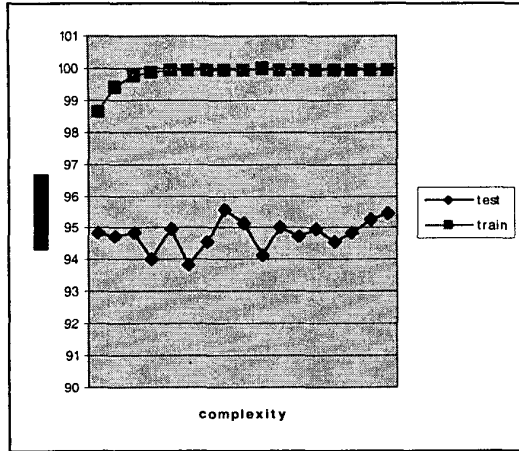
Figure 2. Breast Cancer Wisconsin - no Bagging.
