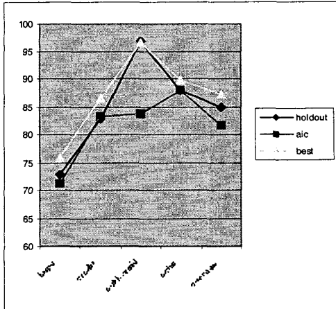
Figure 3. AIC vs holdout vs optimal test set accuracy.
