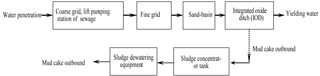
Figure.1 The diagram of XINDU wastewater treatment technology process flow
