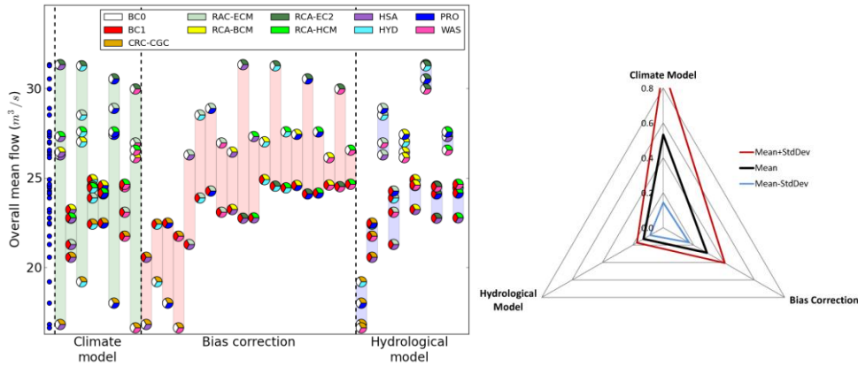
Figure 3: Disparity by model chain component (left) and relative contributions to this disparity (right) of past mean flow for the Loisach river.
