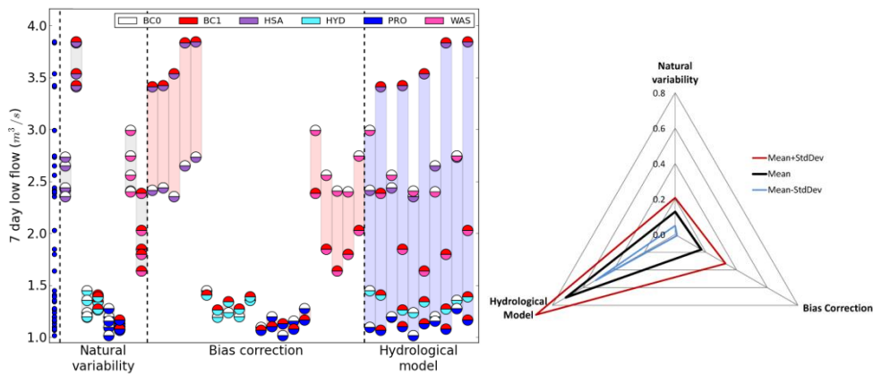
Figure 4: Disparity by model chain component (left) and relative contributions to this disparity (right) of 7-day low flow magnitudes for the Au Saumon river.
