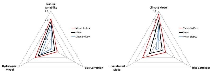
Figure 5 Relative contributions to the uncertainty for the projected change of overall mean flow in the Au Saumon (left) and Loisach (right) rivers.
