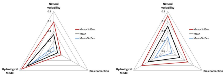
Figure 6: Relative contributions to the uncertainty of 7-day low flow (left) and high flow (right) change in magnitude for the Au Saumon river.
