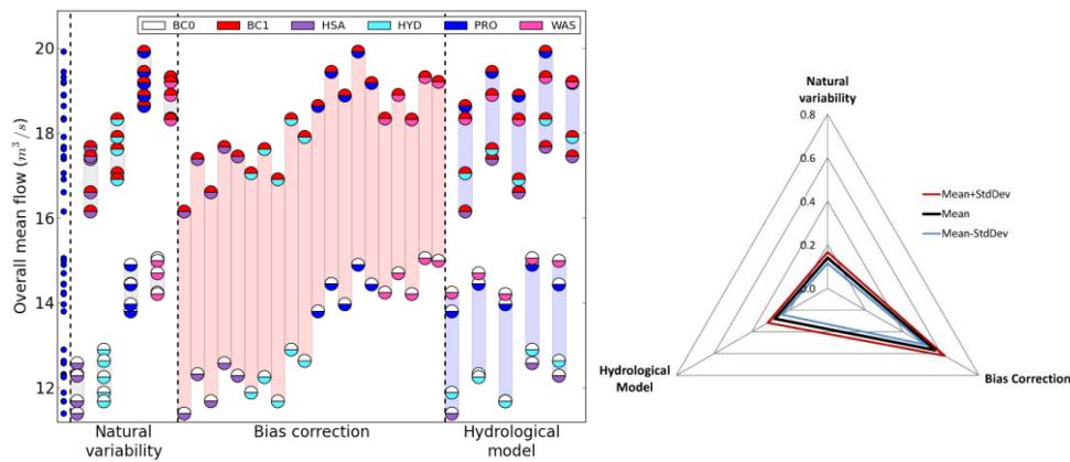
Figure 2: Disparity by model chain component (left) and relative contributions to this disparity (right) of past mean flow for the Au Saumon river.
