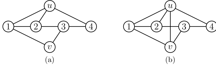
Figure 2.2: Graphs in Example 3.
