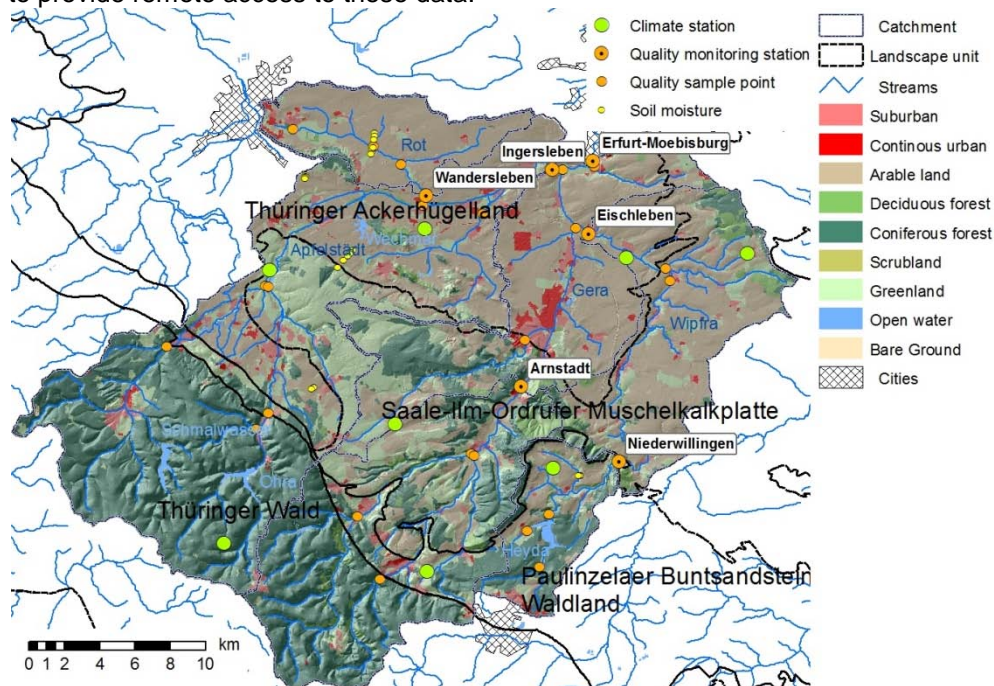
Figure 2. Landscape forms and land-use types in the upper Gera catchment and measurement network of the upper Gera catchment.
