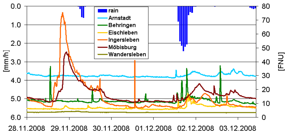
Figure 4. Turbidity of all online stations and average rain (right Y-axis) from 28 th November to 3 rd December 2008.
