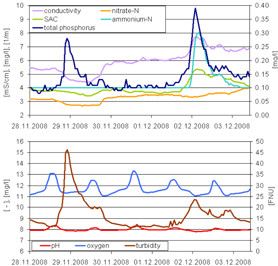
Figure 3. Conductivity, spectral absorption coefficient (SAC), total phosphorous, nitrate, ammonium (right Y-axis), pH, dissolved oxygen, and turbidity (right Y-axis) of the online station Möbisburg from 28 th November to 3 rd December 2008.
