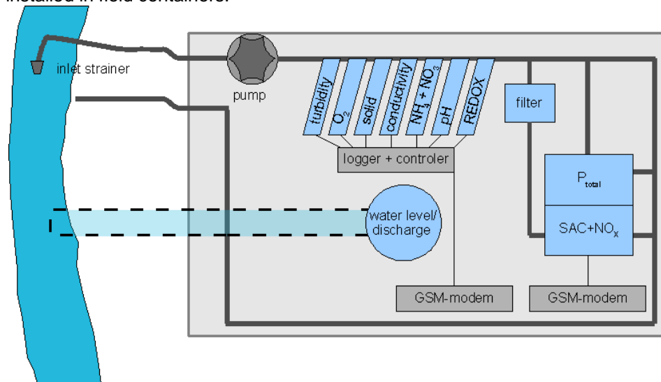
Figure 1. Scheme of the online water-quality stations
