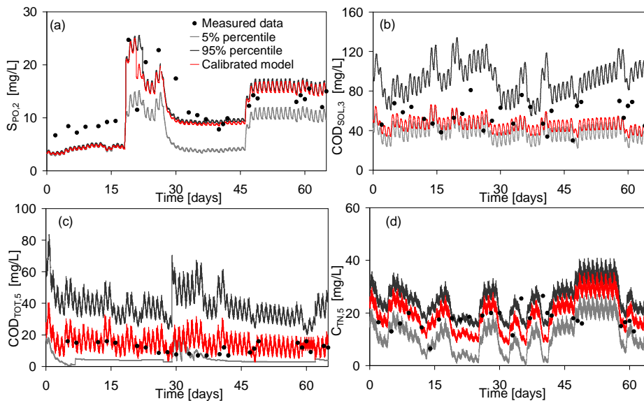
Figure 2 Uncertainty bands, measured data, 5% and 95% percentiles for S_{PO_2} (a), COD_{SOL,3} (b), COD_{TOT,5} (c) and C_{TN,5} (d).
