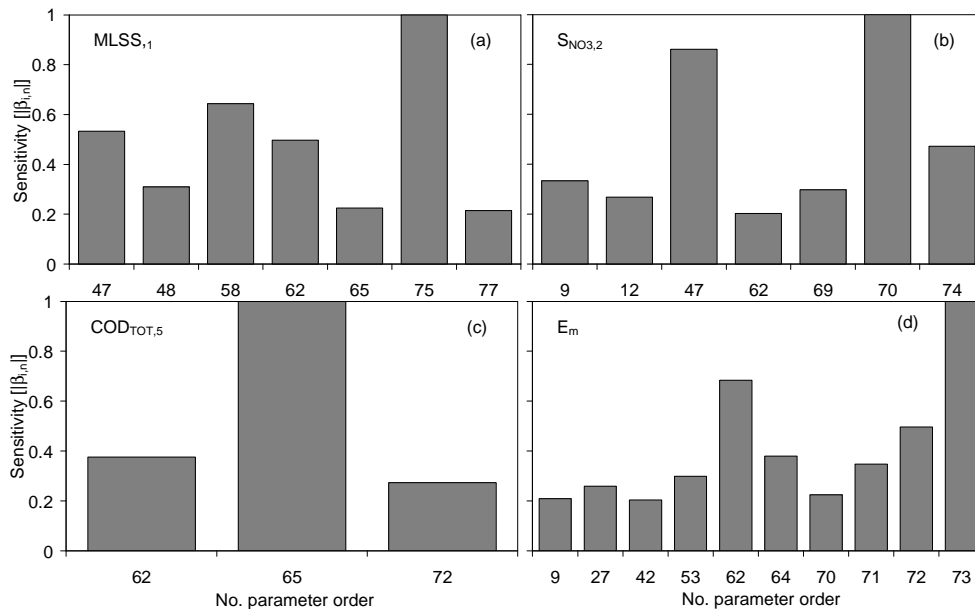
Figure 1 Important model parameters for MLSS_{1,1} (a), S_{NO3,2} (b), COD_{TOT,5} (c) and for E_m (d)
