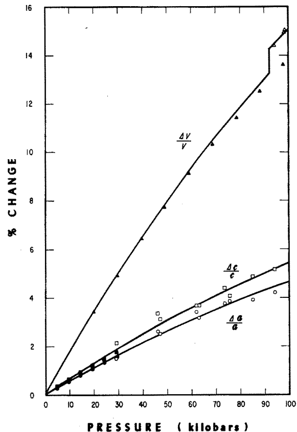
FIG. 2. Linear and volume compressions for Sn (at 25°C) to 100 kbar compared with Bridgman's data. \circ measured a -axis compressions; \square measured c -axis compressions; \bullet Bridgman's a -axis compressions, Ref. 16; \blacksquare Bridgman's c -axis compressions, Ref. 16; \blacktriangle Bridgman's volume compressions, Ref. 17; \triangle measured volume compressions for Sn II phase. The solid lines are quadratic expansions using initial slopes from elastic constants data as discussed in text.
