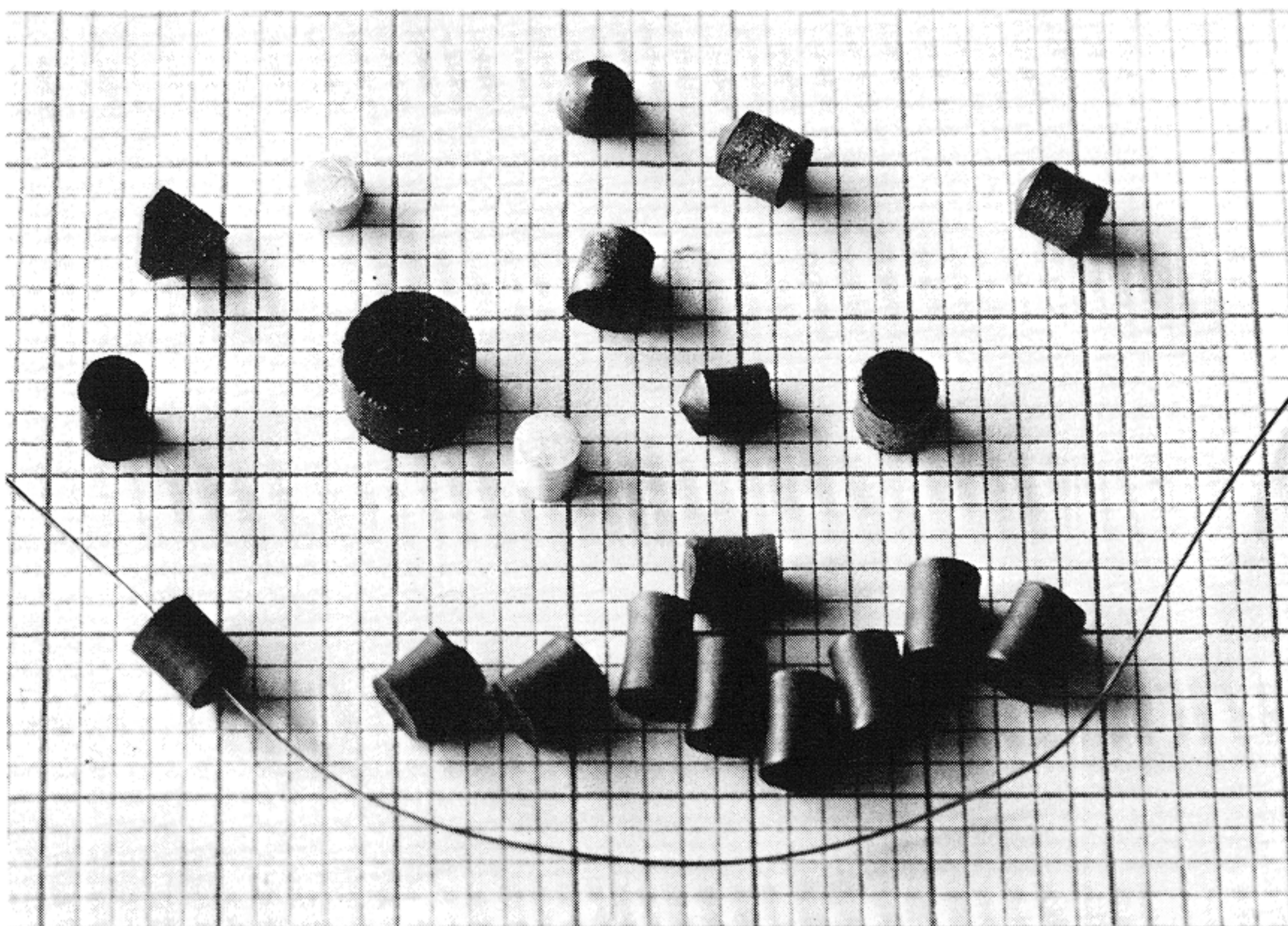
Fig. 1. Sintered diamond shapes (background: 5 squares per centimeter).
