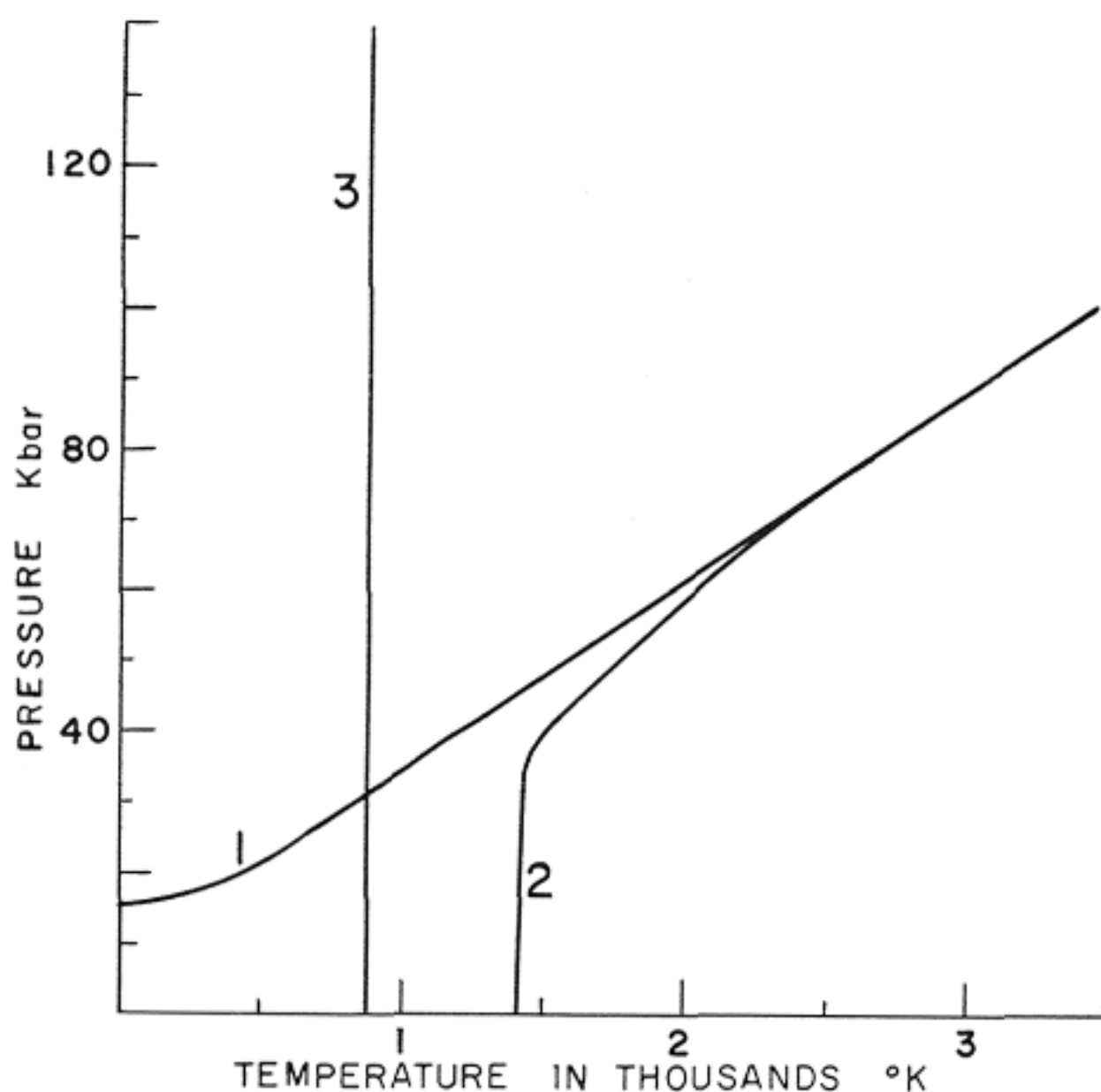
Fig. 2. Diamond sintering regions. Line 1 is the thermodynamic equilibrium boundary for diamond and graphite. Line 3 is a somewhat arbitrary minimum practical sintering temperature for diamond particles. Line 2 is the metastability line for conversion of diamond powder to nondiamond carbon. The location of line 2 depends on time, but the form of the curve for other time periods is similar to the 30-minute curve which is shown.
