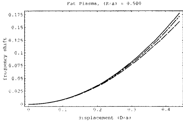
FIG. 6. Frequency shifts for a fat plasma ( R/a = 0.500 ) with a sharp boundary and with a diffuse boundary compared to the empirical fit. The solid curve is the sharp boundary case. The diffuse boundary case is the dashed curve. The empirical fit curve of Fine et al. lies between (dot-dashed). The vertical scale is significantly reduced compared to Figs. 4 and 5 indicating a flattening of the curves as they approach the origin. As R/a increases further, both the empirical fit and our calculations predict the onset of a negative frequency shift for small D/a . The grid used is 101 \times 101 .
