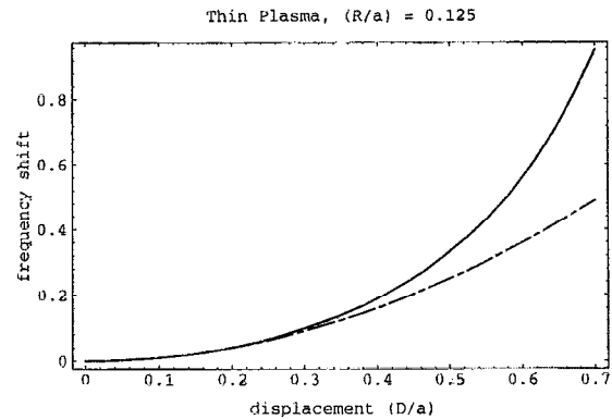
FIG. 4. Frequency shifts for a thin plasma ( R/a = 0.125 ) with a sharp boundary and with a diffuse boundary compared to the empirical fit. The curves for sharp and diffuse boundaries are virtually identical (solid line) and the lowermost curve (dot-dashed) at top right is the empirical formula of Fine et al. The grid used is 101 \times 101 .
