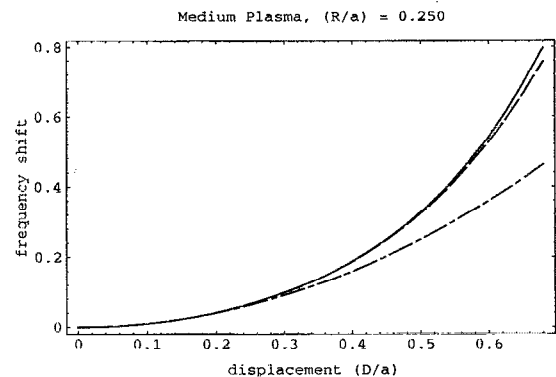
FIG. 5. Frequency shifts for a medium-size plasma ( R/a = 0.250 ) with a sharp boundary and with a diffuse boundary compared to the empirical fit. The solid curve is the sharp boundary case, the dashed curve is the diffuse boundary case, and the dot-dashed curve is the empirical formula of Fine et al. The grid used is 101 \times 101 .
