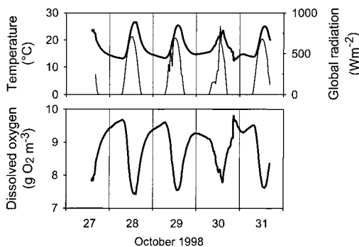
Fig. 1. Top: Surface water temperature (bold line) in the main channel of the Hassayamapa River and global radiation (fine line) at Wickenburg airport. Bottom: Dissolved oxygen concentration in the surface water of the main channel.
