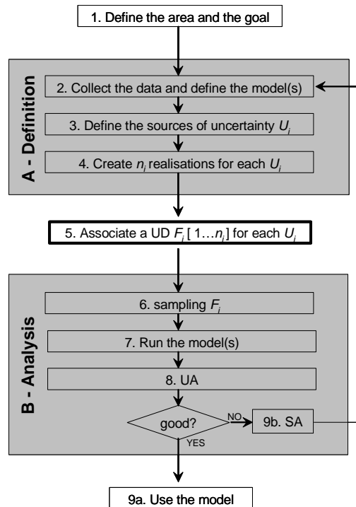
Figure 1. Flowchart of the General Probabilistic Framework (GPF).
