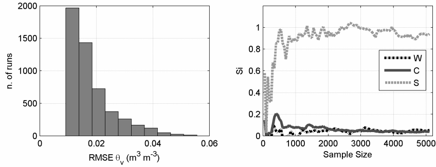
Figure 2. Histograms of the RMSE calculated between simulated and measured mean soil moisture \theta_v (-) and sensitivity indexes.
