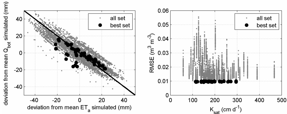
Figure 4. correlation between the deviation from the mean of evapotranspiration ( ET_a ) and bottom fluxes ( Q_{bot} ) (left); scatter plot of K_{sat} and RMSE (right).
