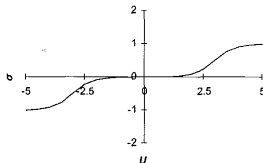
Figure 6. Improved activation function with stable region around 0.
