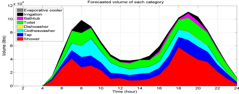
Figure 6 Disaggregation of predicted 24-hour water demand
