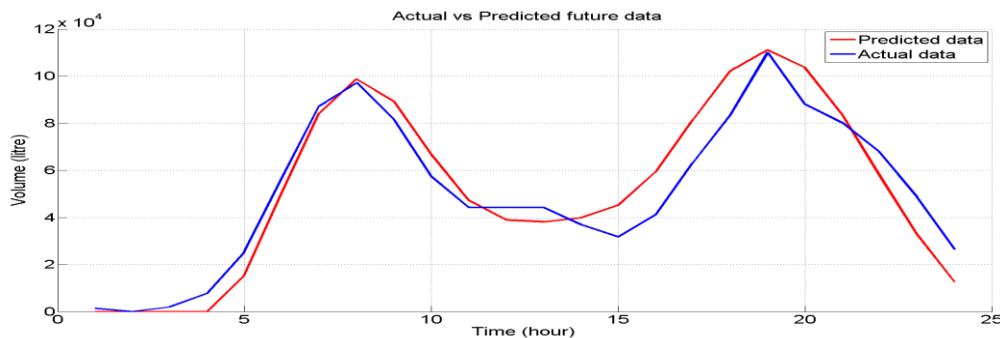
Figure 4 Actual vs predicted water consumption
