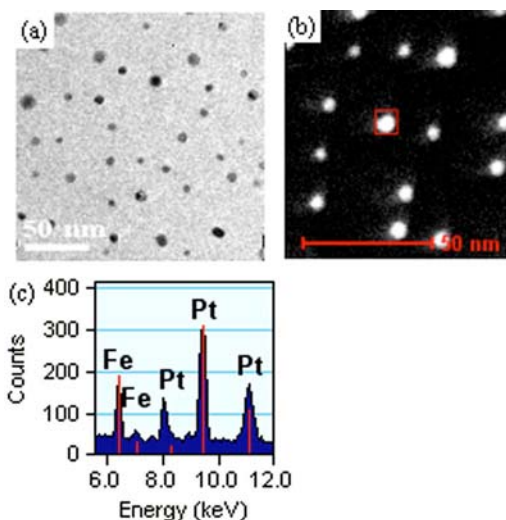
FIG. 2. TEM image and EDX spectrum of indicated individual FePt nanoparticle for sample B.
