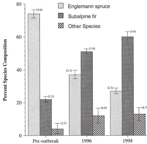
Fig. 2. Percent species composition pre-outbreak, 1996, and 1998, \pm standard error of the means ( \pm s.e. ). Other species includes aspen, Douglas-fir, and limber pine.
