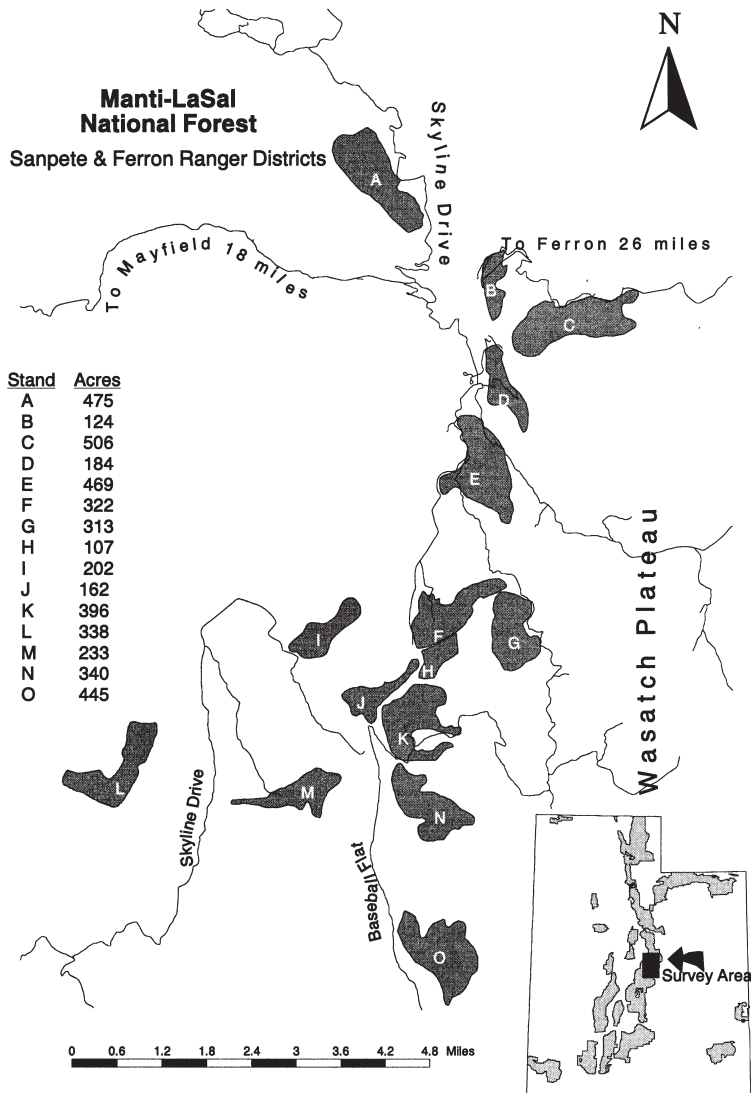
Fig. 1. Map of Wasatch Plateau, Manti-LaSal National Forest, Utah, showing Engelmann spruce stands surveyed to determine spruce beetle-caused impacts. Acres of each stand are also represented.
