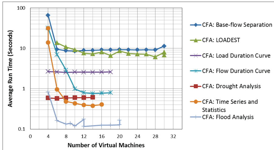
Figure 2. Load Testing Results 2-4 requests/s
