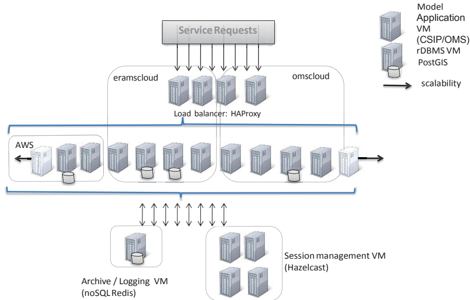
Figure 1. CSIP Physical Architecture.
